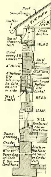
Wall Section
